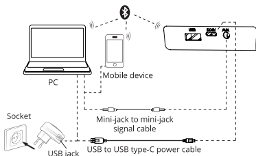
Fig. 2. Connection diagram
