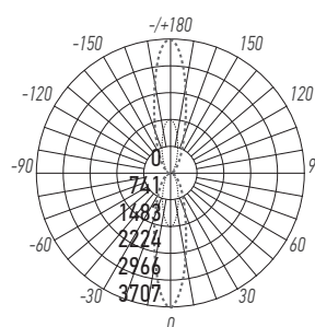
PWL-300110/30D 2x9w
