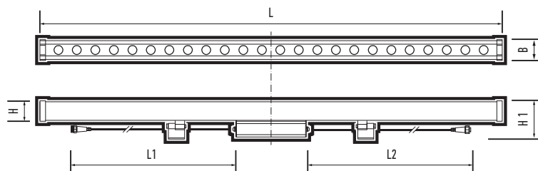
PWW 1000
