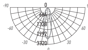
PWL-200110/30D 1x9w
