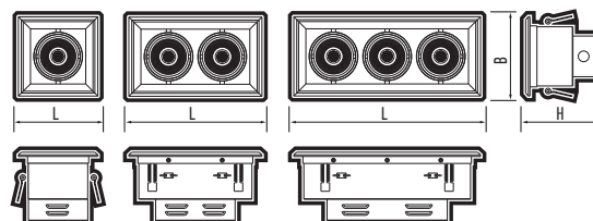
PSP-S 311 1x9w
