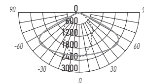
PGL 03 60w
