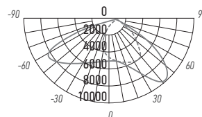
PSL 08 150w 140/70°
