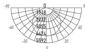
PFL-C3 150w
