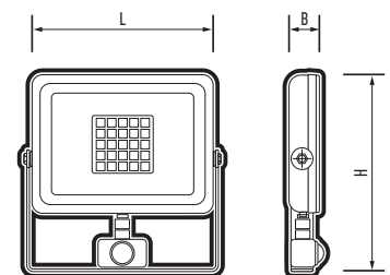
PFL-SC SENSOR
