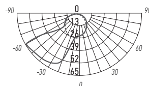
PWS/R R5060
